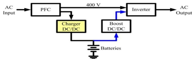
Fig. 1. Proposed UPS system
