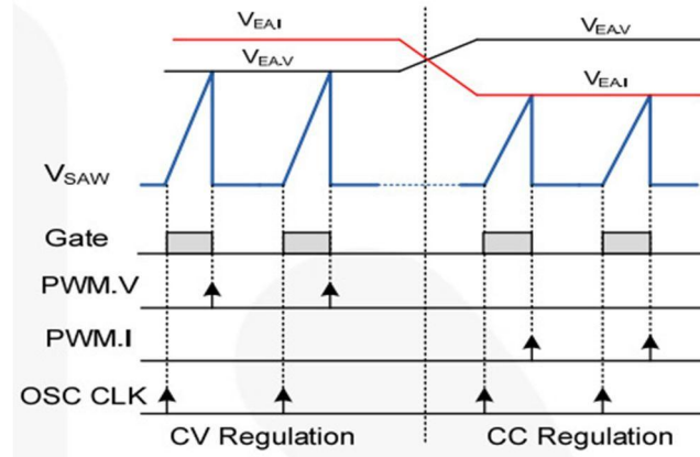
Fig. 7. PWM Operation for CV and CC Modes
